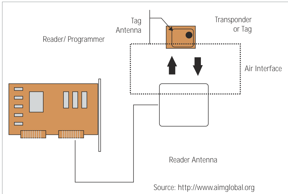
Figure 1: RFID system components
